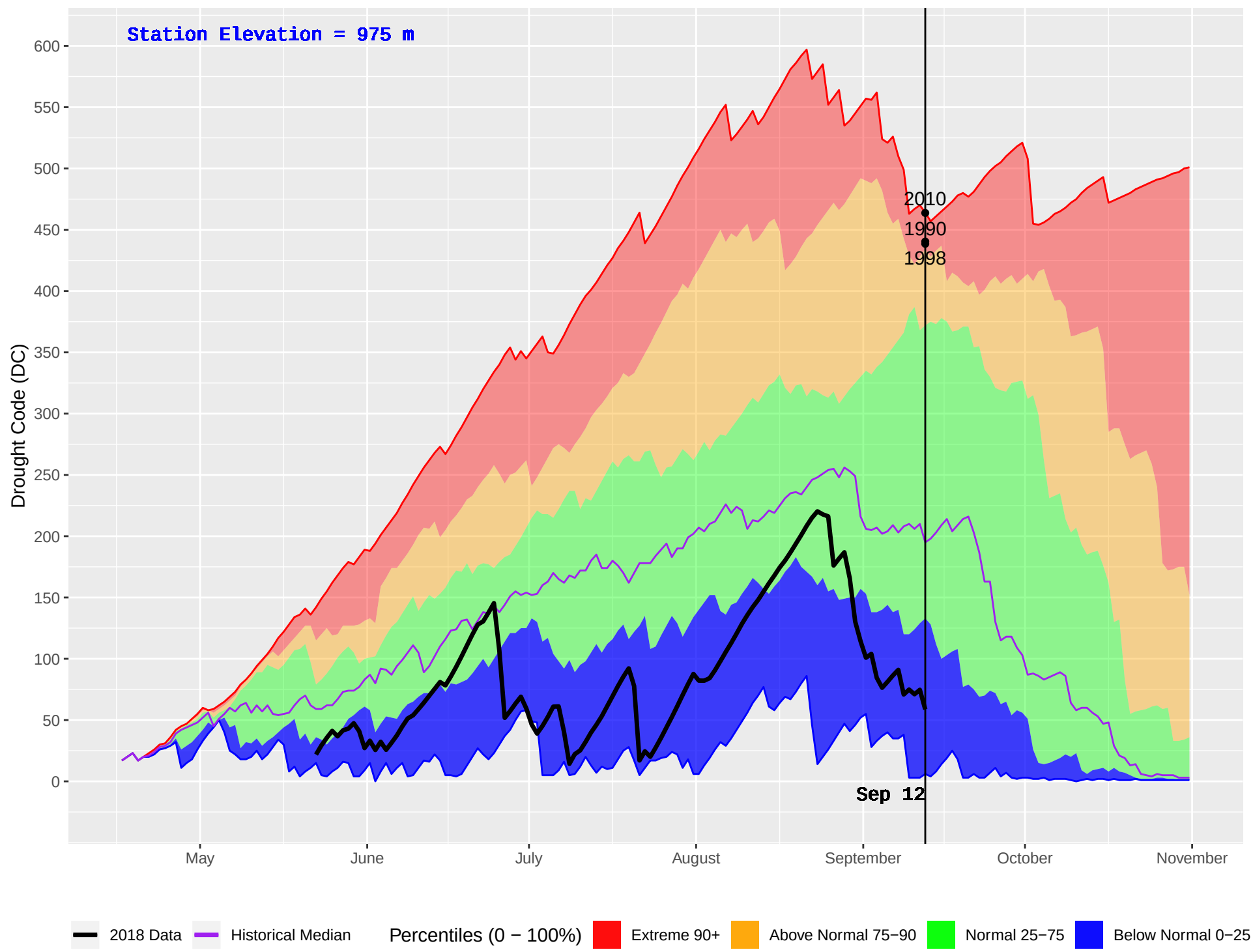
MCGREGOR 2 (192) : Historical (1986–2016) and Current (2018) Daily Drought Code (DC)
